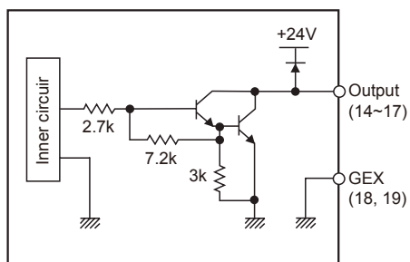
< CN3 control output connections >
